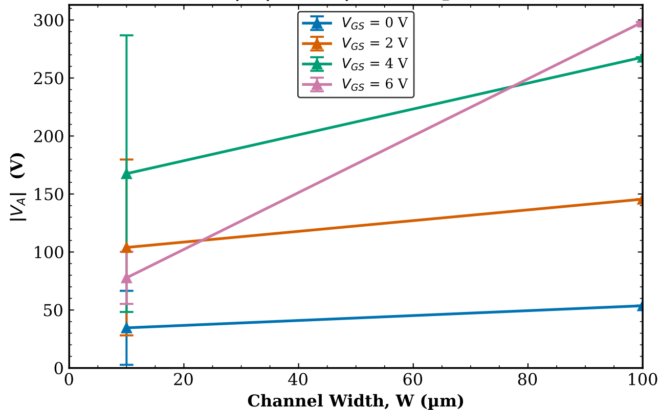
TFT3 Combined (Tr. 1 & 2) |V_A| vs W | L = 80\text{ }\mu\text{m}
